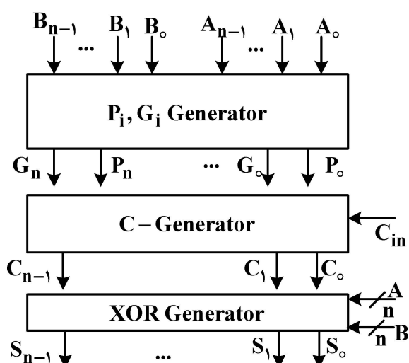
P_i, G_i Generator
